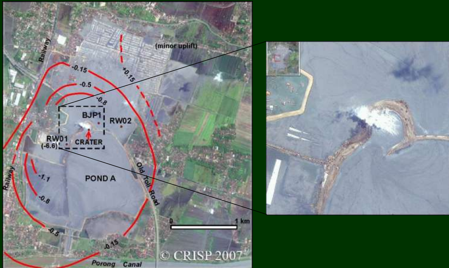
Satellite photo (05.06.07) of the LUSI MV with subsidence contours (m/yr) from INSAR data one year after the eruption.
